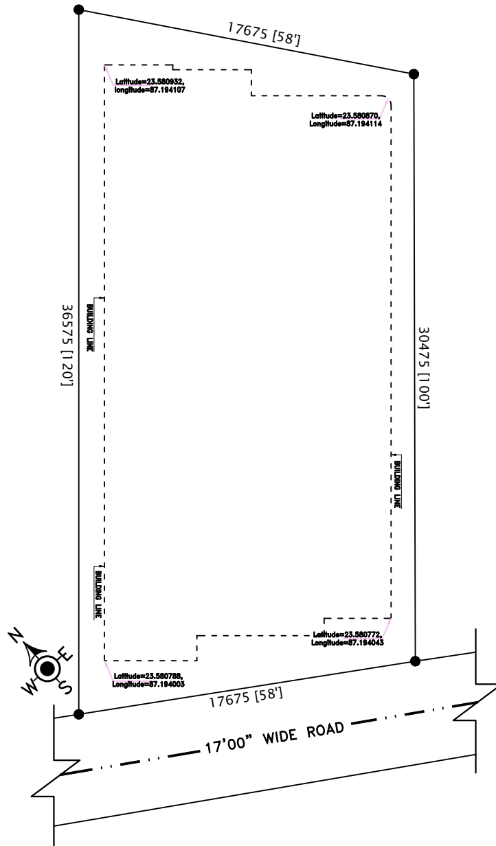
(A) SITE PLAN SCALE: 1:100
